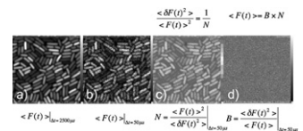
Figure: a) Fluorescence image of B. subtilis cells expressing GFP. b) Image taken with a laser dwell time faster than the diffusion time of a GFP molecule. c) Number map determined from fluctuations at each pixel from 50 fast images. Color scale is from 0 to 18 molecules. d) Brightness map determined from (a) divided by (c).
